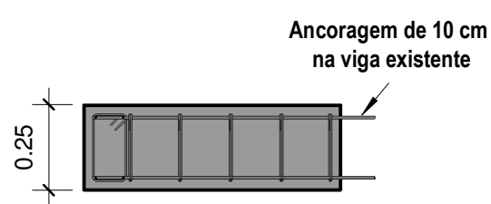
12 Concreto V6=V7 - Central GLP 1 : 20
